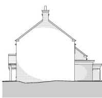
East Elevation
